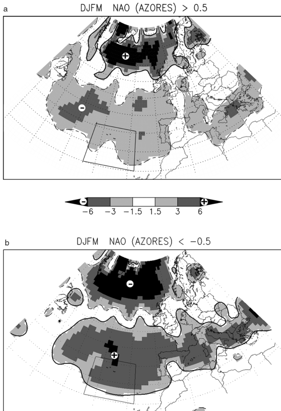
Figure 5 Number of cyclones per winter (DJFM), detected within boxes of 5^\circ longitude \times 5^\circ latitude and normalized for 50^\circ N (period 1958–2000). (A) NAO > 0.5; (B) NAO < -0.5. NAO index defined between Ponta Delgada (Azores) and Stykkisholmur (Iceland)
