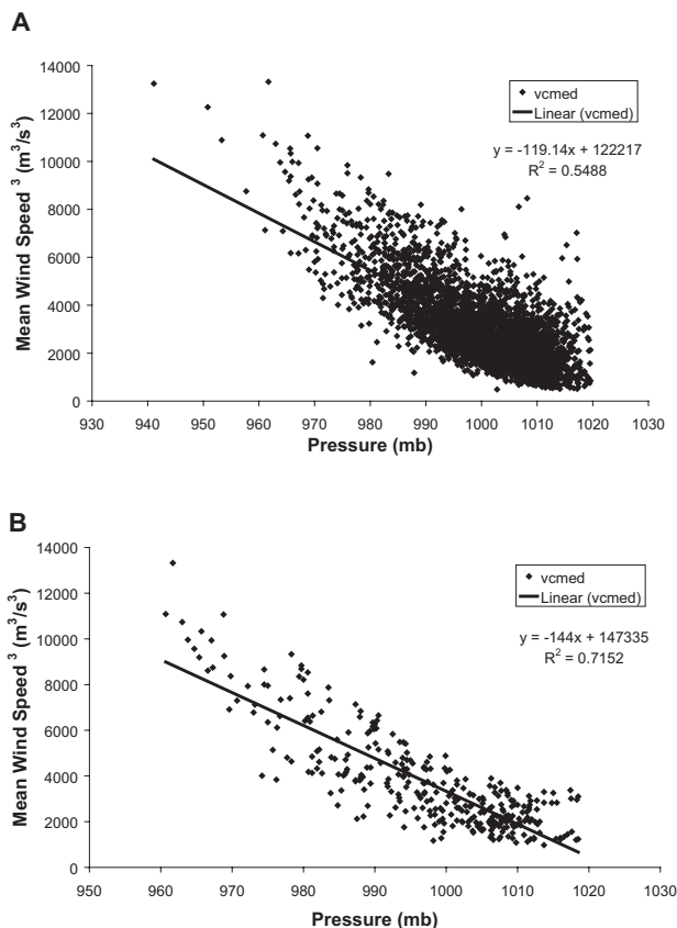
Figure 4 (A) Relationship between pressure and the spatial average of the cube of wind speed (vcmed) for all the cyclones in the work region for the 1958–1998 period. (B) The same as in (A) but only for the cyclones that affected the Azores Islands according to the documentary record. The linear regression line is also represented in both figures (Linear vcmed)
