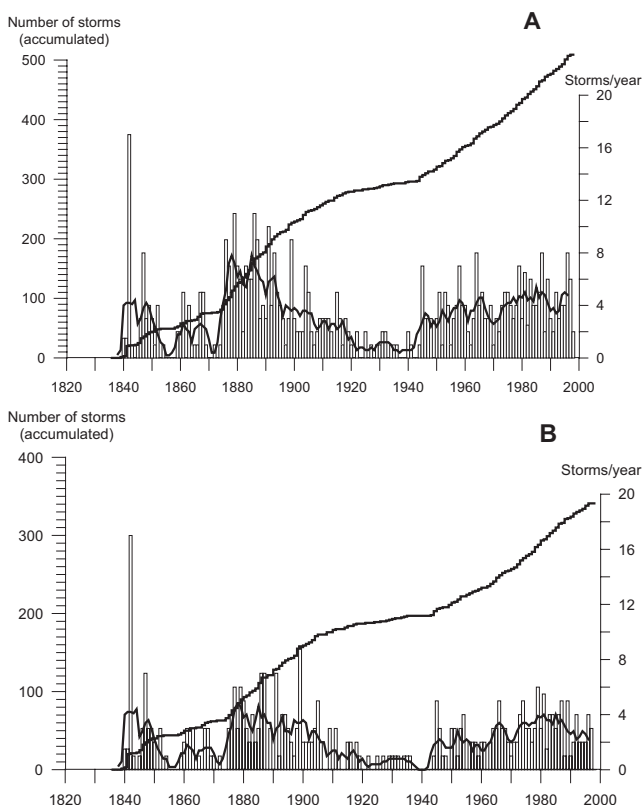
Figure 3 Bar charts of storm frequency, 5-yr running means and step plot of accumulated frequency of storms. (A) Series III; (B) series IV
