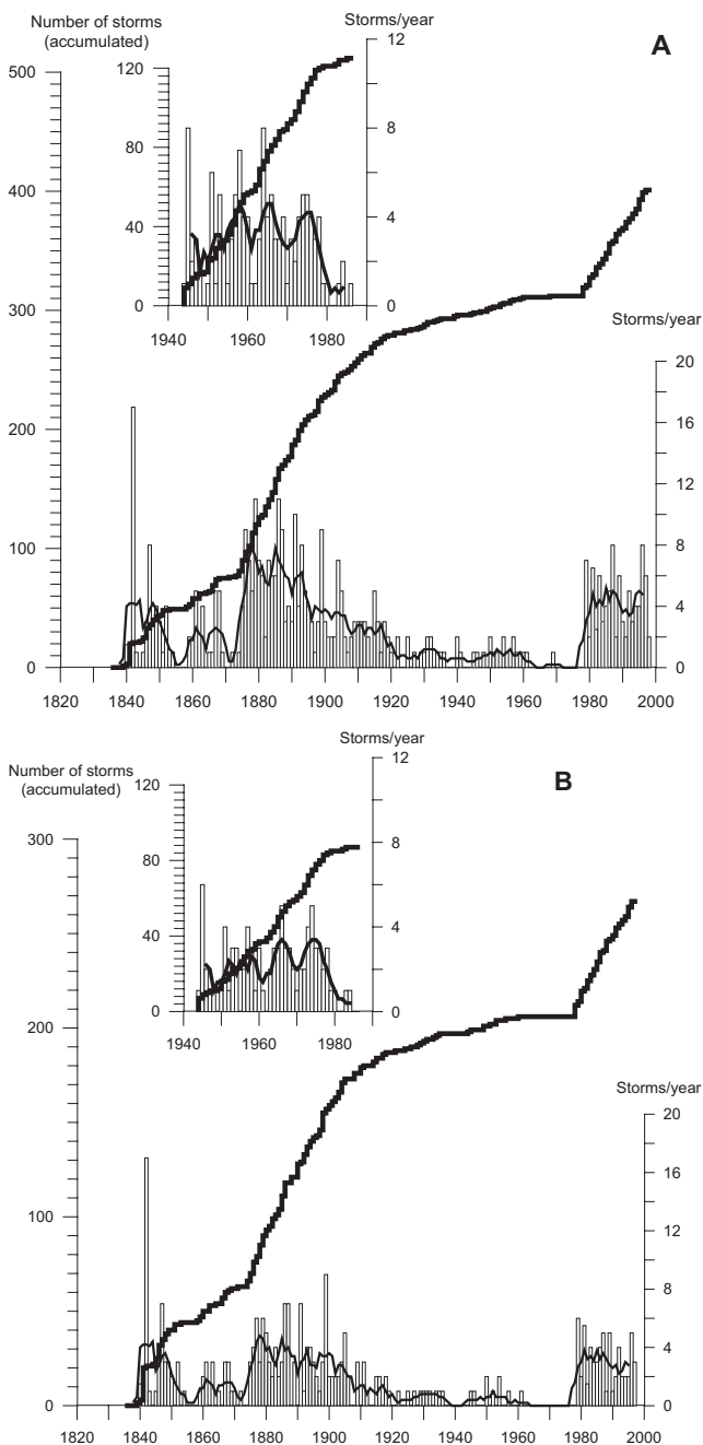
Figure 2 Bar charts of storm frequency, 5-yr running means and step plot of accumulated frequency of storms derived from the newspaper Açoriano Oriental (AOR). (A) Series I; (B) series II. Insets: equivalent information derived from the newspaper Açores (ACR)
