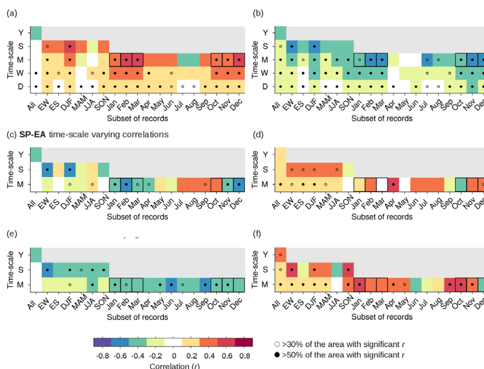
Figure 1. Temporal correlation ( r ) between modes (NAO ((a), (b)), EA ((c), (d)) and SCAND ((e), (f)) indices) and resources (SP ((a), (c), (e)) and WP ((b), (d), (f))) at various time-scales and considering various subsets of records of the whole series. Daily (D), weekly (W), monthly (M), seasonally (S) and yearly (Y) averaged series are considered (y-axis), when possible (EA and SCAND indices are only available at the monthly and longer time-scales). In each case we have considered all the records in the series (All), but also, when it makes sense (when not colored in gray), only those records corresponding to each one of the four seasons (winter, i.e. DJF; spring, i.e. MAM; summer, i.e. JJA; and autumn, i.e. SON), and only those corresponding to each one of the twelve months (from January to December). This is indicated in the x-axis. The series of SP and WP considered are spatially averaged series involving those land grid points within the IP where the correlation between the indices and the resources is significant ( p < 0.05 ). An empty (solid) circle denotes that the size of this area represents more than a 30% (50%) of the whole land area of the IP. Black squares indicate the case studies that were further investigated.
